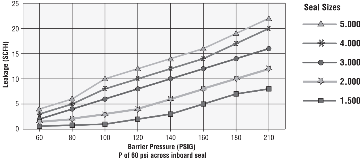
Type 7828G Estimated Total Barrier Gas Consumption
