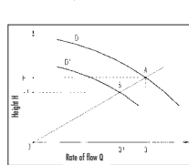
Diagram to determine turning diameter.
