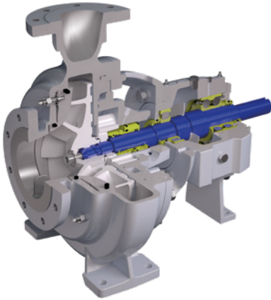
Liquid ring pump LM
