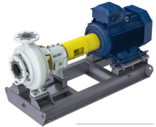
Heavy-duty baseplate
